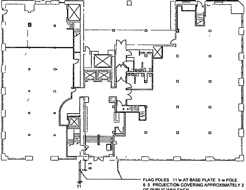
1 FIRST FLOOR PLAN 1" = 20'-0" 0 10 20 60
