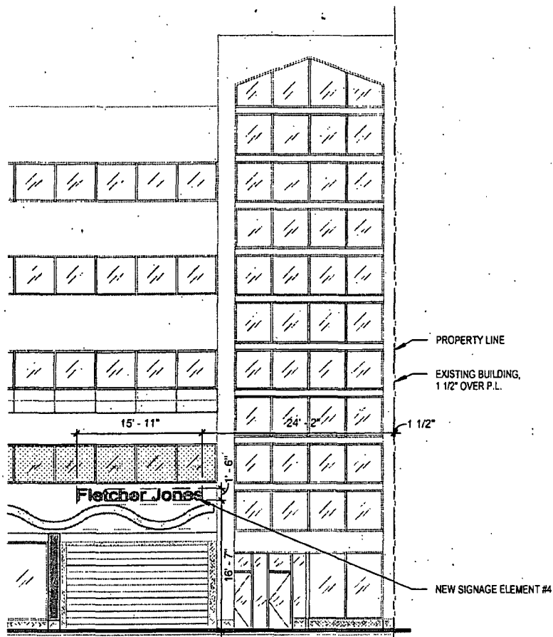
ELEVATION - EAST
