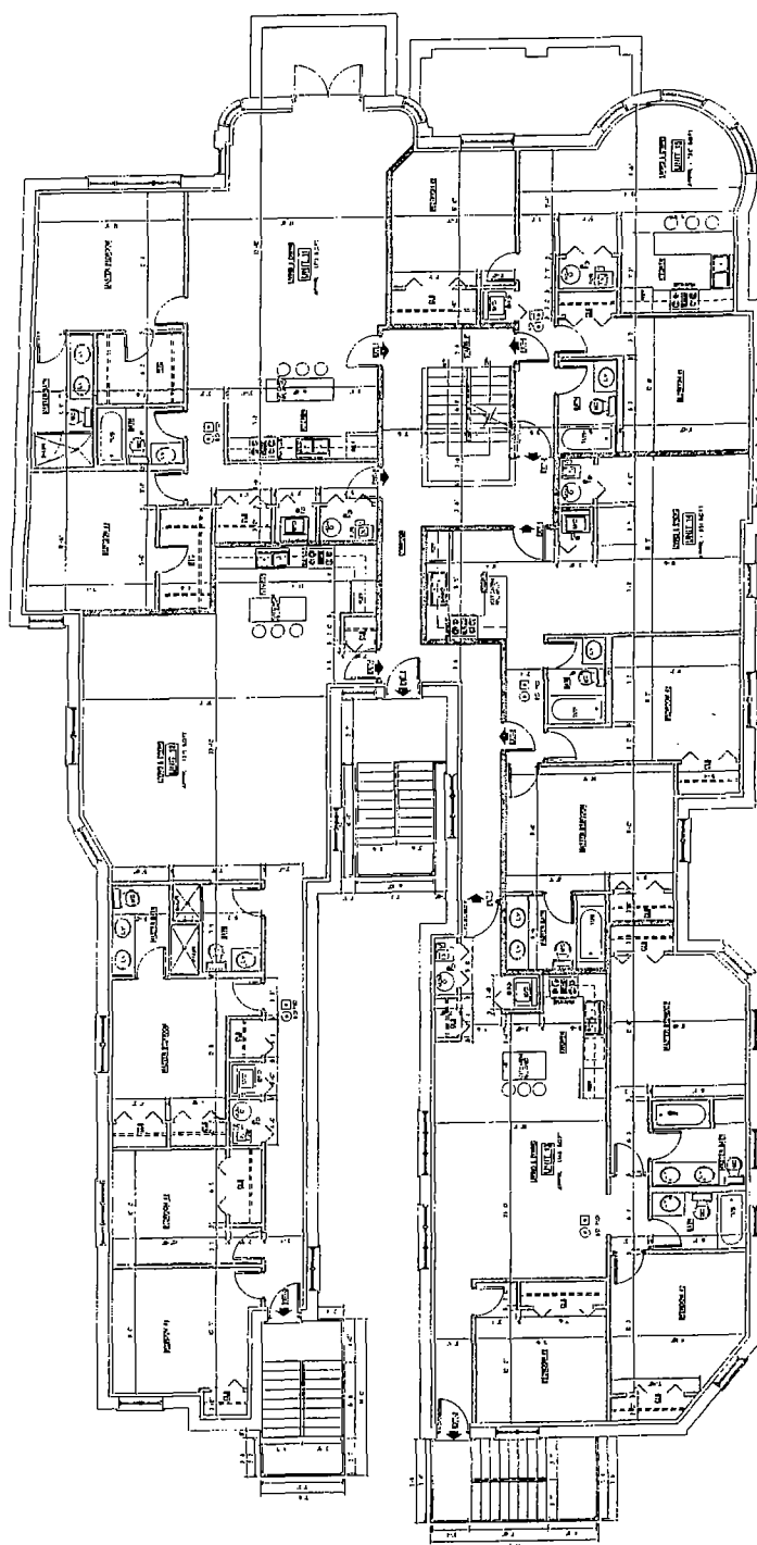
TYP FLOOR PLAN SCALE 3/16" = 1'-0"
