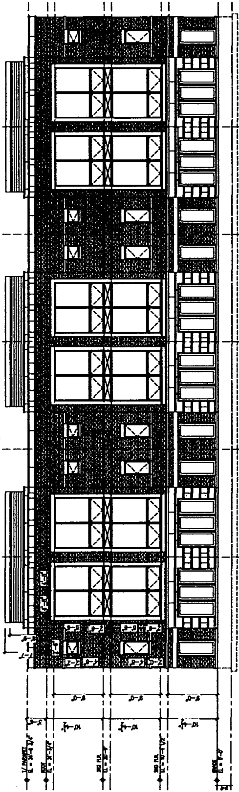
1 FRONT ELEVATION A2.0 3/16"=1'-0"
