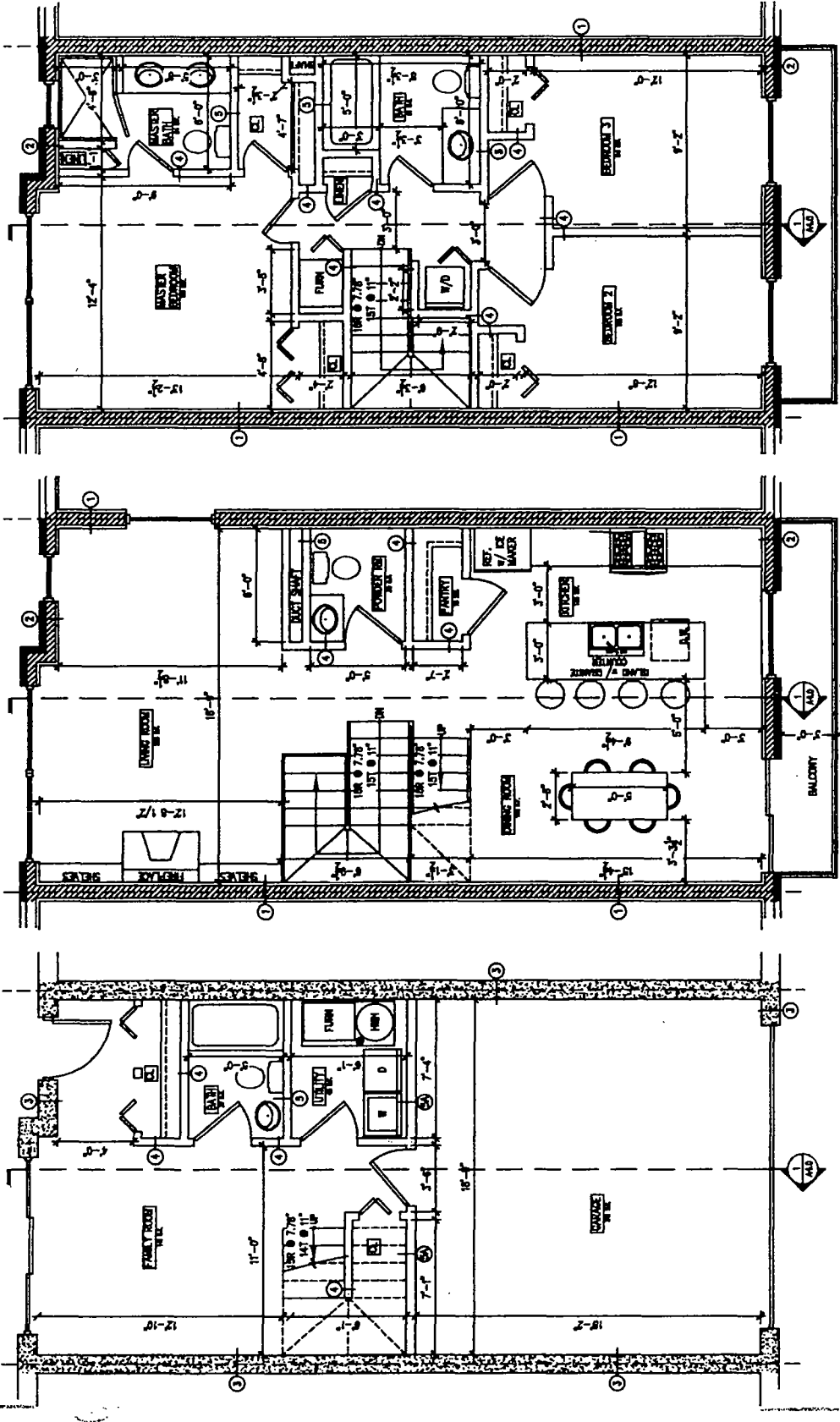
1 FIRST FLOOR PLAN A1.1 3/8"=1'-0"
