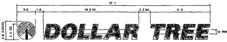
42 LOGO 36 DOLLAR TREE Face L/R Channel Ltrs / RW SCALE 1/4" = 1'-0"
