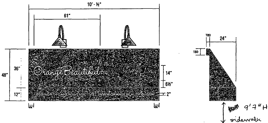
A Non-Illuminated Awning - 1" Aluminum Tube Frame • Front View SCALE 3/8" = 1' 0" • For Production / For Presentation
