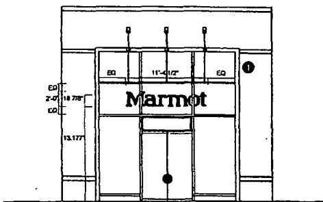
Front V. ew SCALE: 1/8" = 1'-0"
