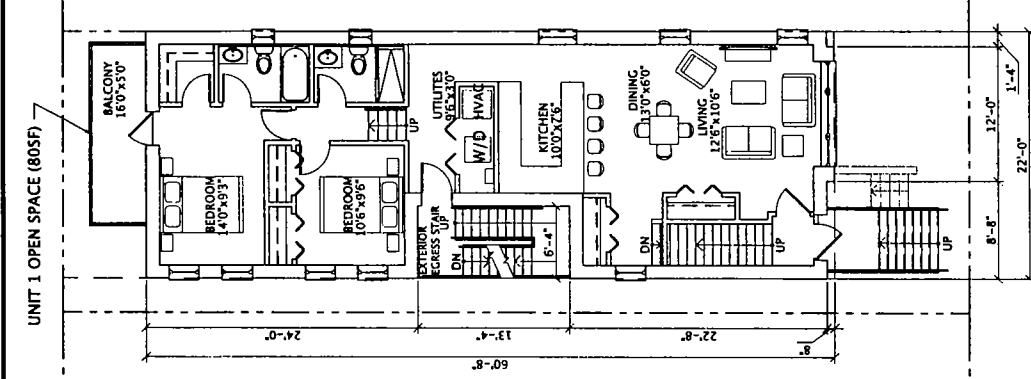
1st FLOOR PLAN - UNIT 1
