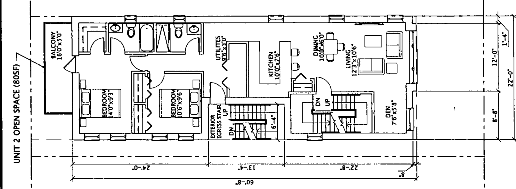
2nd FLOOR PLAN - UNIT 2
