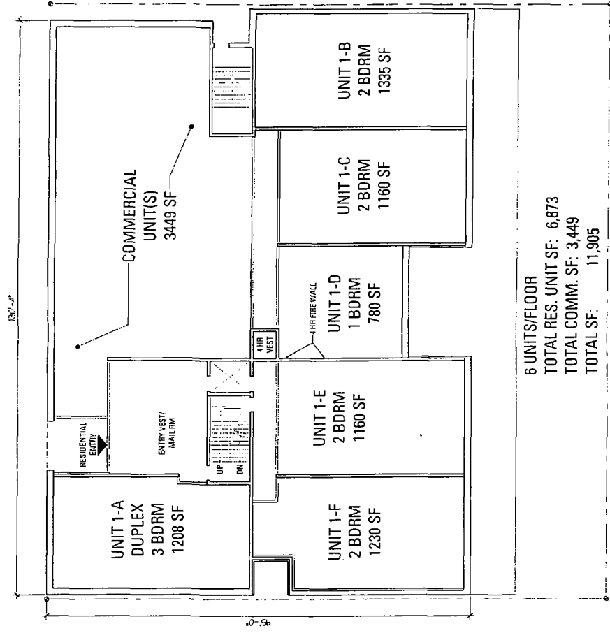
1ST FLOOR/GRADE PLAN 1/16" = 1'-0"
