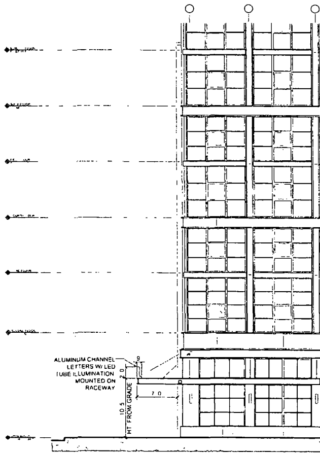
1401-1411 E 53rd ST WEST ELEVATION SIDEWALK
