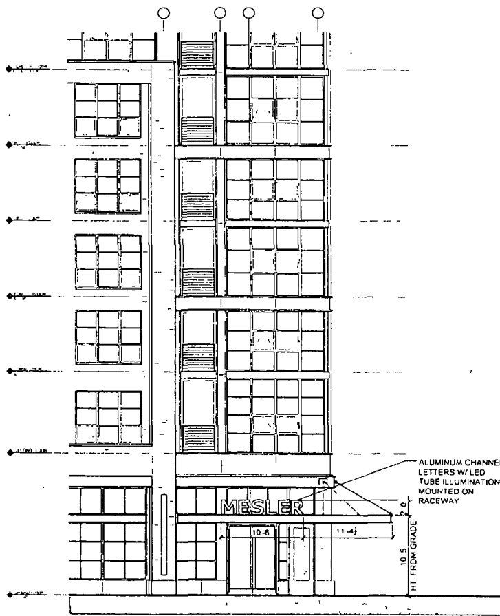
1401-1411 E 53rd ST NORTH ELEVATION
