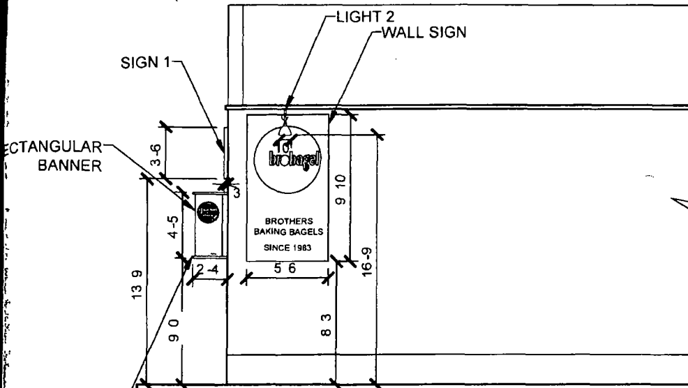
ADJACENT ALLEY ELEVATION 3/32" = 1'-0"
