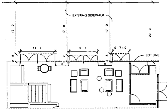
③ UPRW PLAN DETAIL 1/8" = 1' 0"
