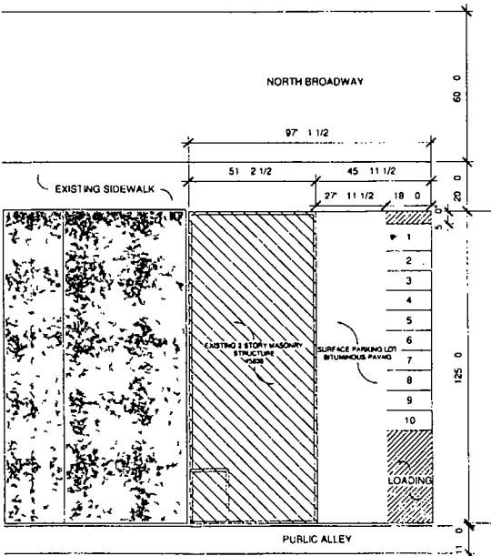
① UPRW SITE DETAIL 1" = 30' 0"
