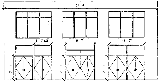
② UPRW ELEVATION DETAIL 1/8" = 1' 0"
