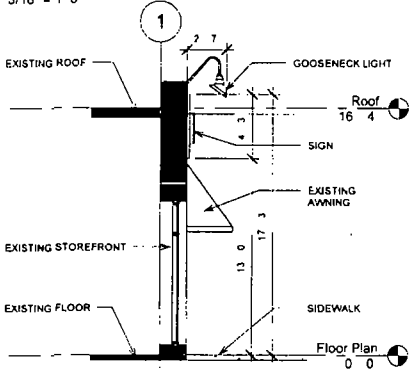
② SIGN SECTION 3/16 = 1" 0"
