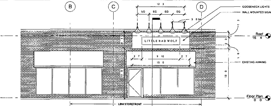
① SIGN ELEVATION 3/16 = 1" 0"
