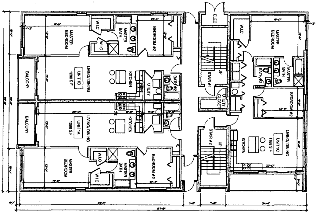
Second Floor Plan Third floor similar
