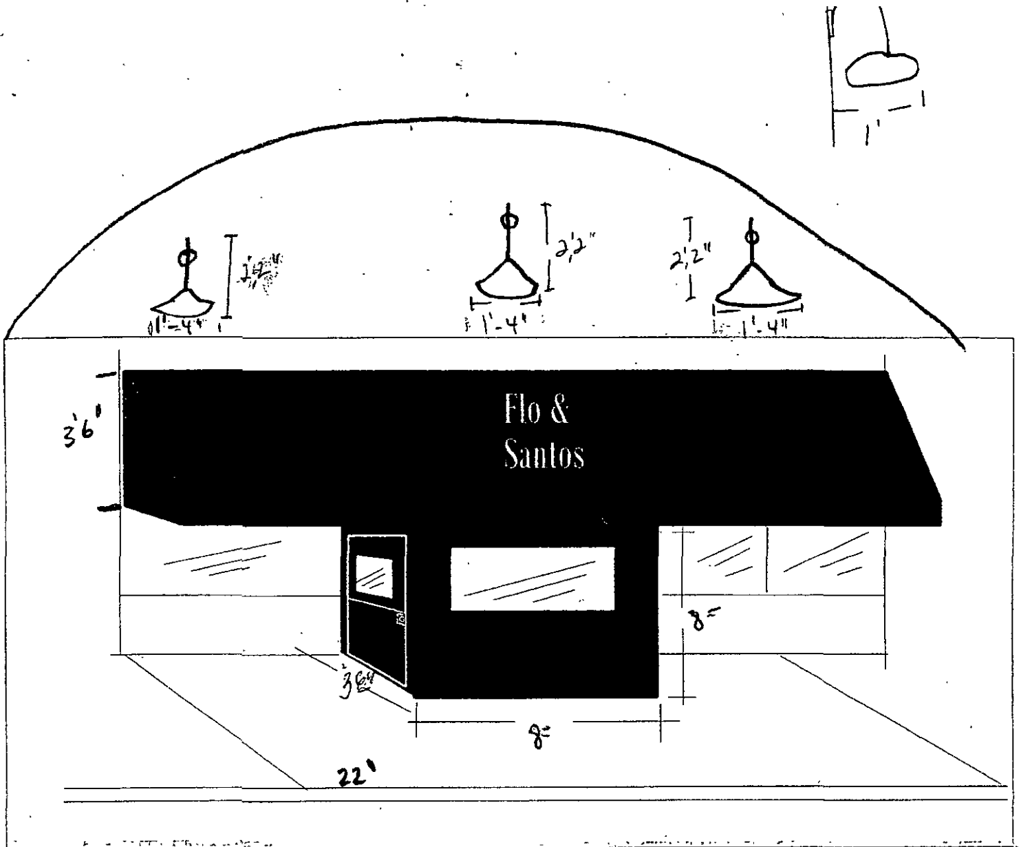
EAST ELEVATION Wabash Facing Front
