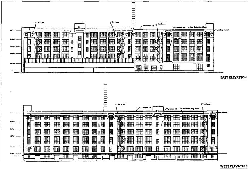
WEST ELEVATION
