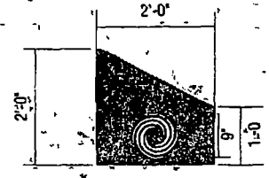
END VIEW DETAIL (1) LOGO ON EACH END
