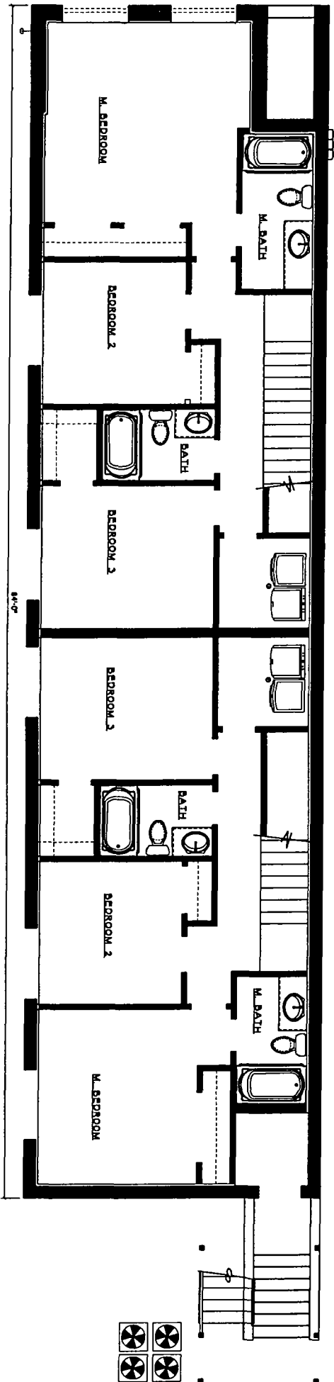
1 BASEMENT PLAN SCALE 1/8" = 1'-0"
