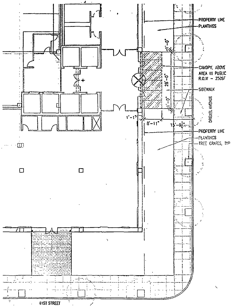
1/16" = 1'-0"
