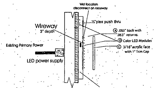
Typical Wireway Mount channel Letters with LED's
