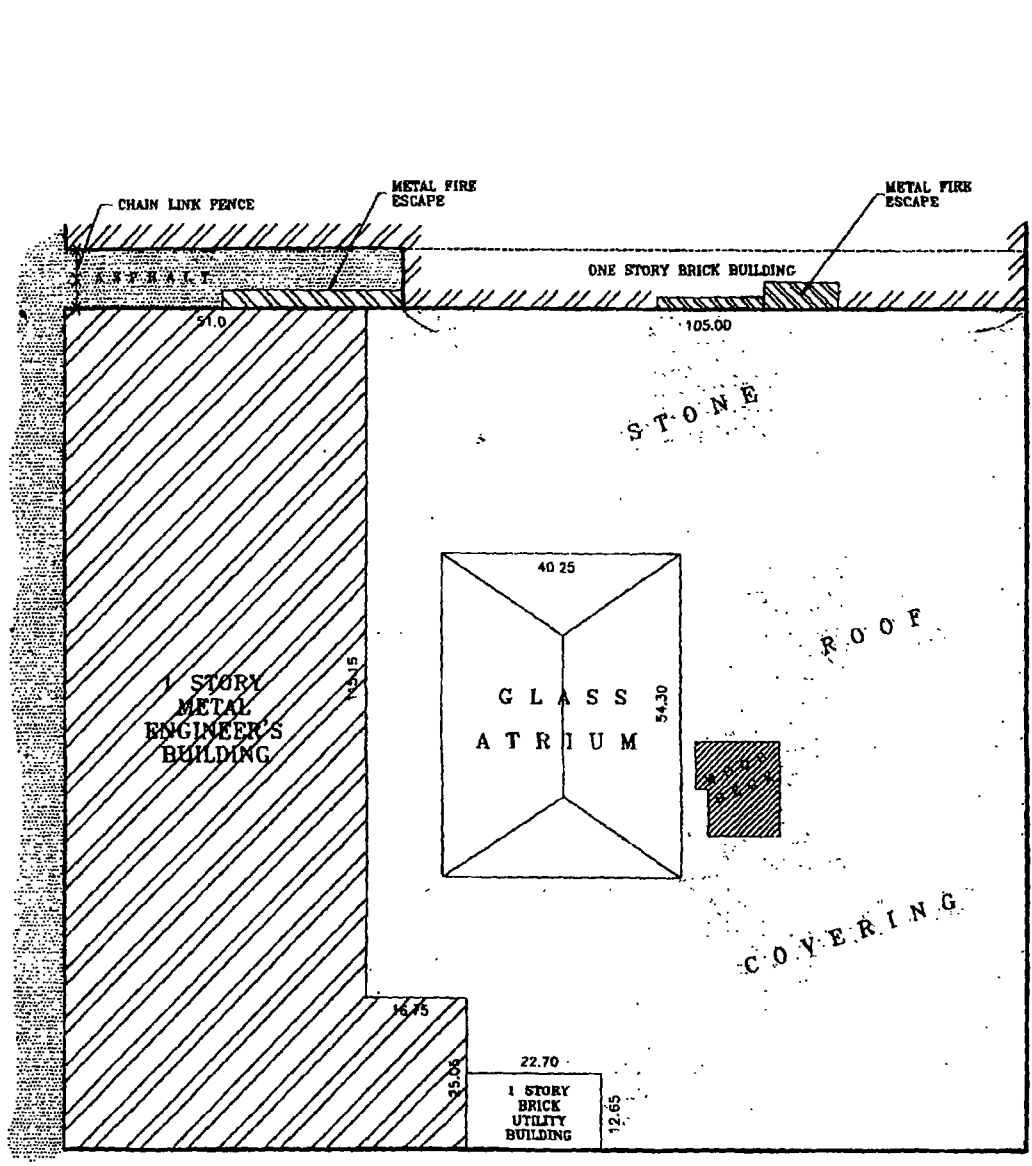
ROOF DETAIL
