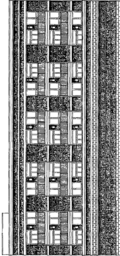
1 North Elevation Scale 1/8" = 1'-0"
