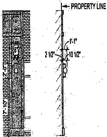
② LIGHT FIXTURE ELEVATION & SECTION - TYPE A 1/8" = 1'-0"
