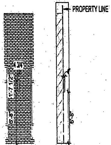
③ LIGHT FIXTURE ELEVATION & SECTION - TYPE C 1/8" = 1'-0"
