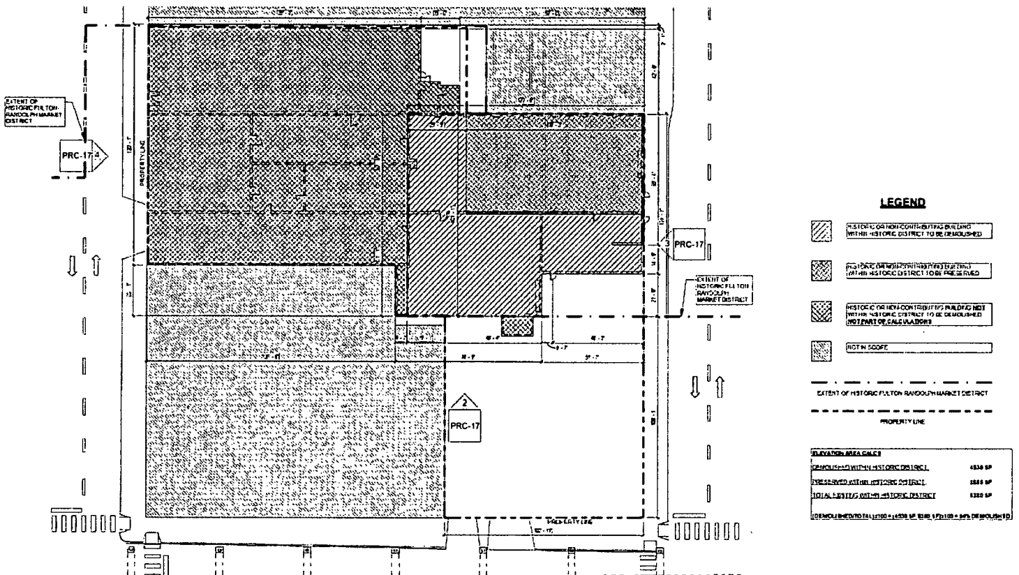
Demolition Plans (Source: NORR and Acosta Ezgur, LLC)
