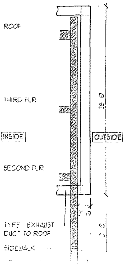
A SECTION 1/8" = 1' 0"
