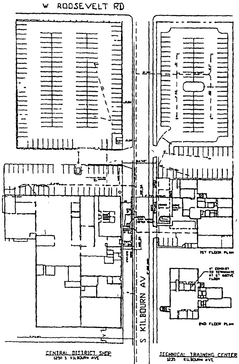
LOCATION PLAN SCALE 1" = 60'
