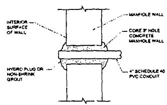
MANHOLE CONDUIT PENETRATION SCALE: NOT TO SCALE
