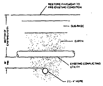
(1) - 4" BORE UNDER EXISTING UTILITIES SCALE: NOT TO SCALE
