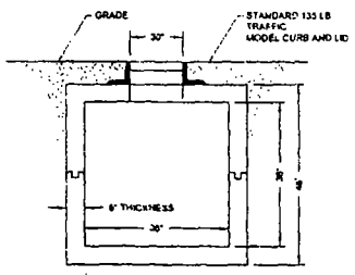
3' X 3' X 3' MANHOLE SCALE: NOT TO SCALE
