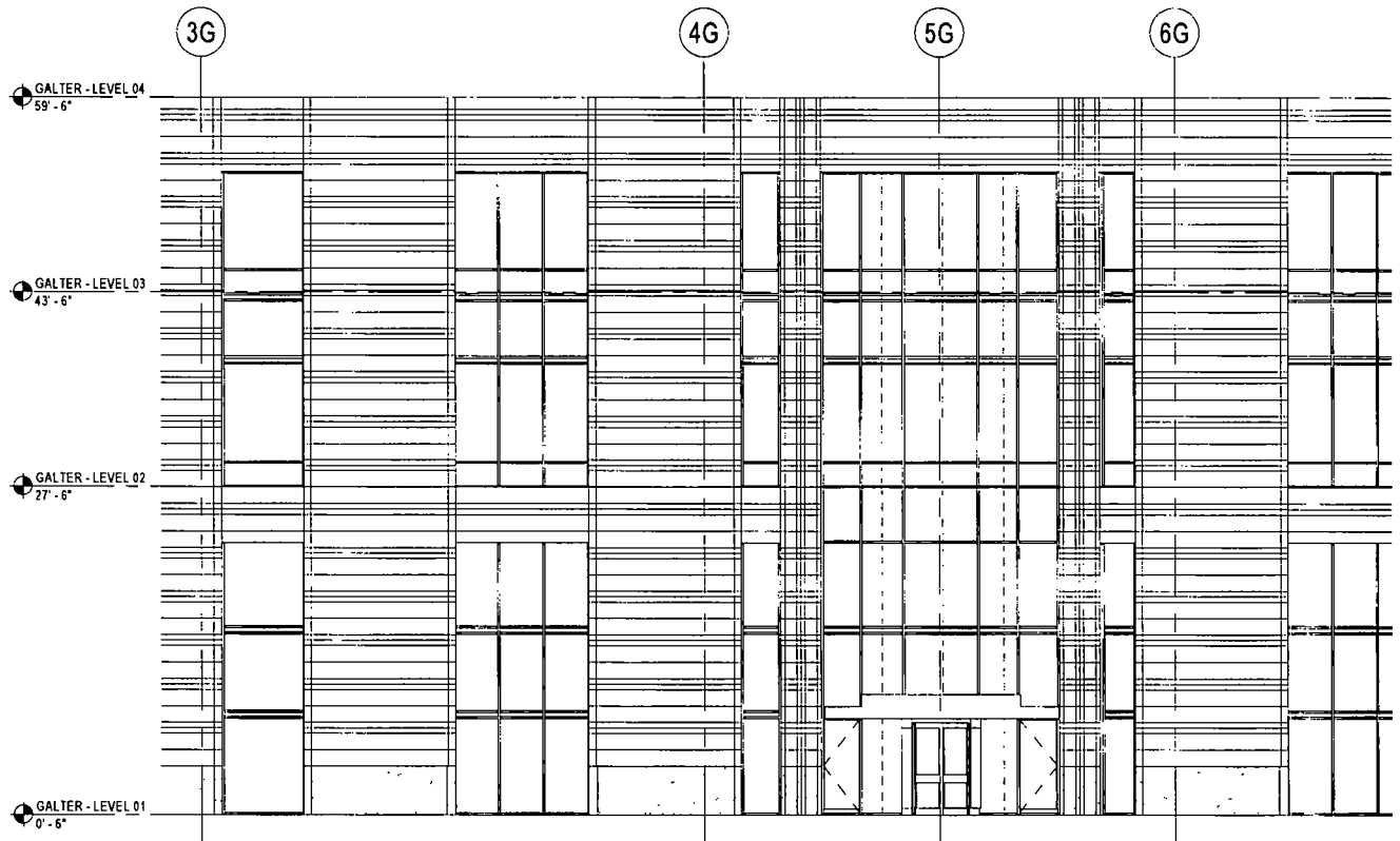
EXISTING ELEVATION FACING NORTH
