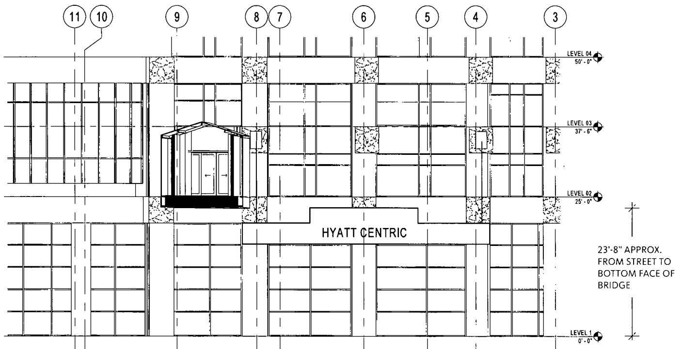
EXISTING ELEVATION FACING SOUTH
