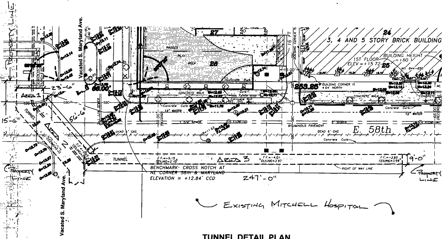
TUNNEL DETAIL PLAN
