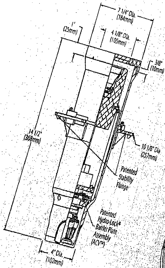
SIDE VIEW
