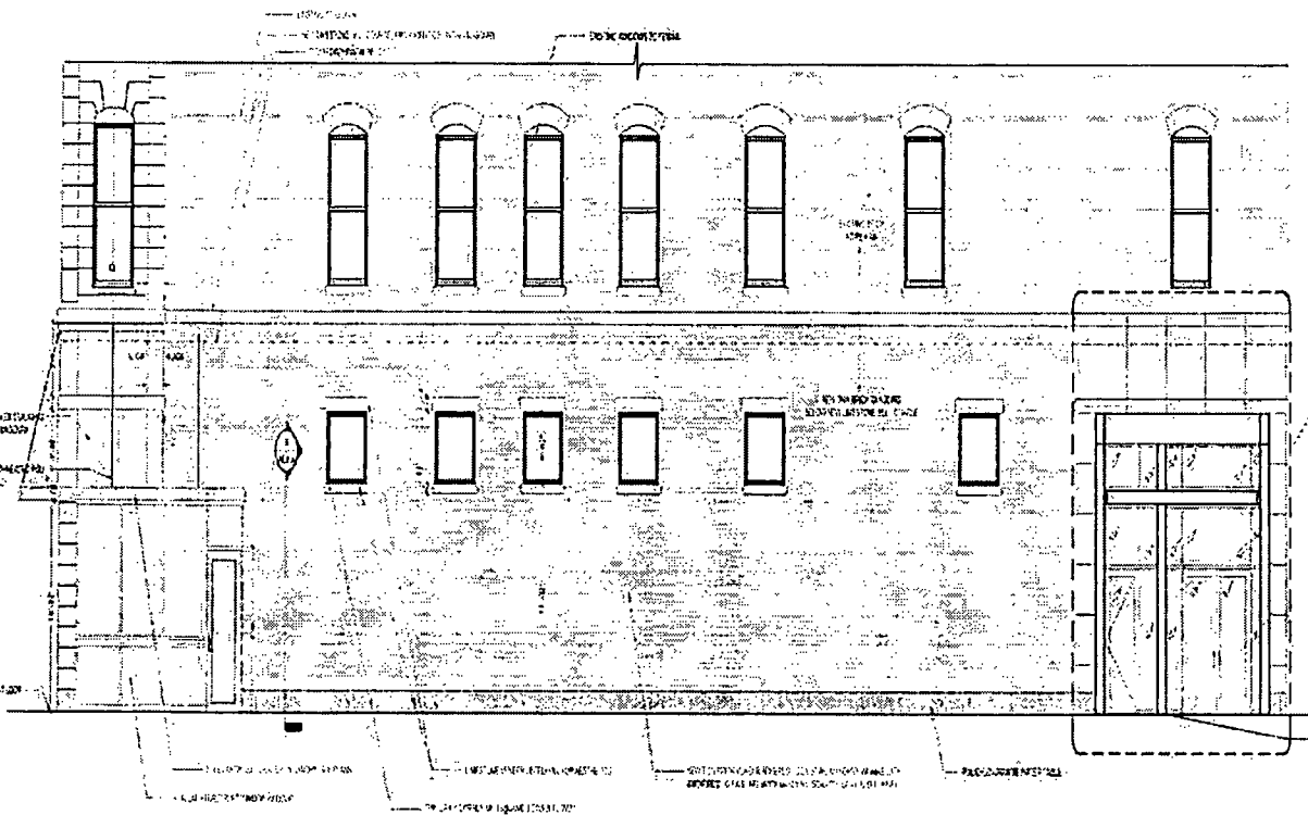
① EXTERIOR ELEVATION - NORTH 1/4" = 1'-0"
