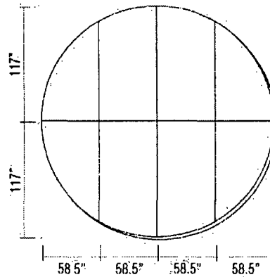
FRONT CONSTRUCTION VIEW
