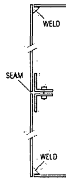
SIDE VIEW MAGNIFIED / NOT TO SCALE
