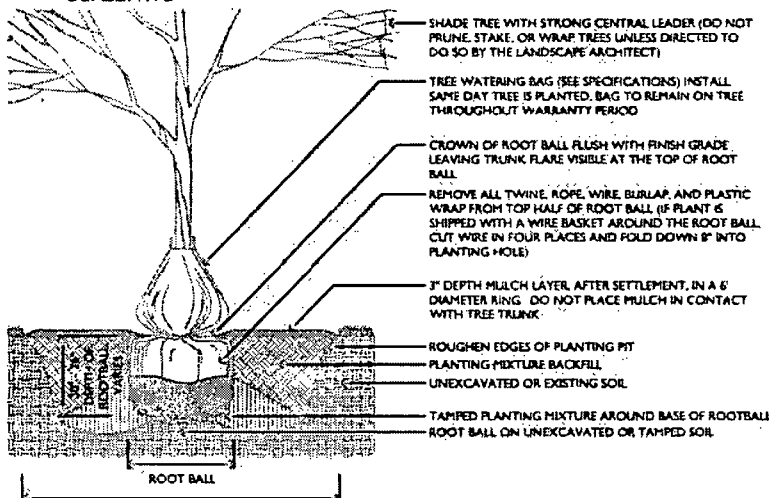
2 TREE INSTALLATION DETAIL
