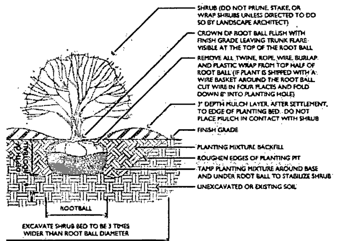
3 SHRUB INSTALLATION DETAIL
