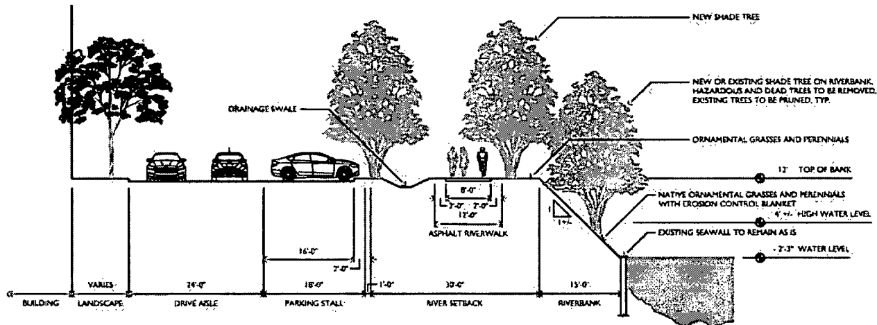
RIVERBANK AND RIVER SETBACK SECTION
