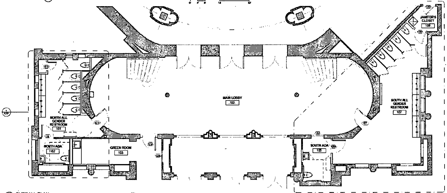
1 OVERALL PLAN WF 11/17
