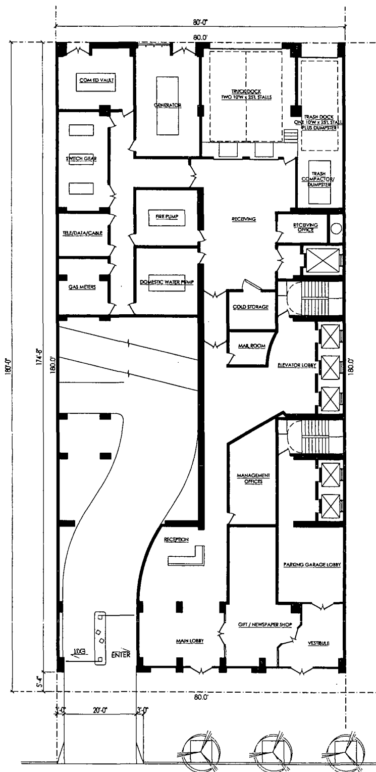
PROPOSED GROUND FLOOR / SITE PLAN - 14,055 SF
