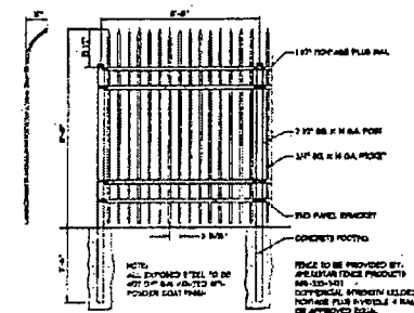
1 PROPOSED 6' HT. SECURITY FENCE FOR 63RD ST. FRONTAGE NOT TO SCALE
