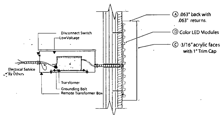
Typical Flush Mount Channel Letters with LED's
