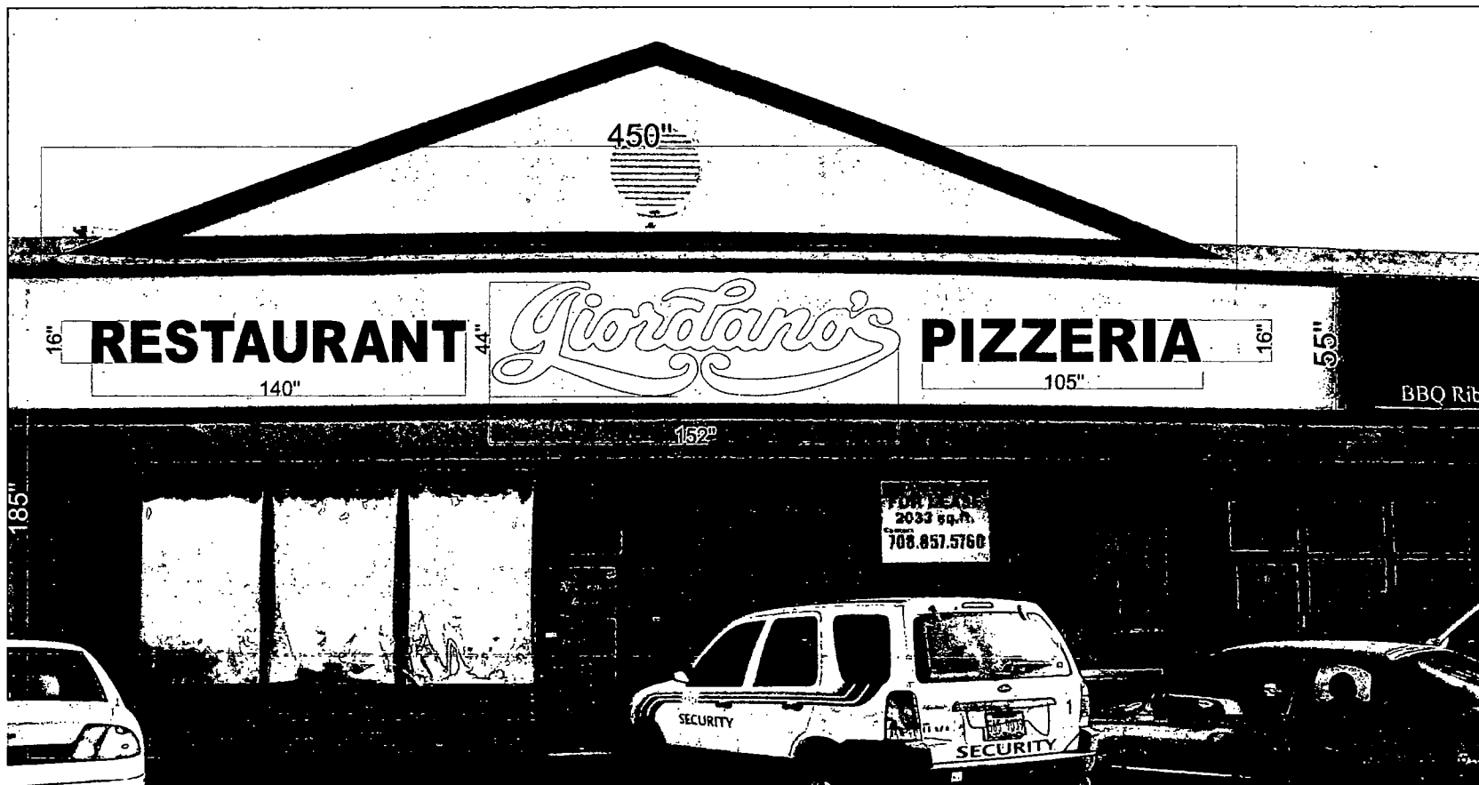
Typical Flush Mount Channel Letters with LED's
