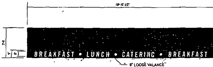
B AWNING ELEVATION DETAILS SCALE 3/8" = 1'-0"
