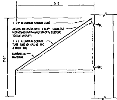
SECTION @ AWNING SCALE 1" = 1'-0"
