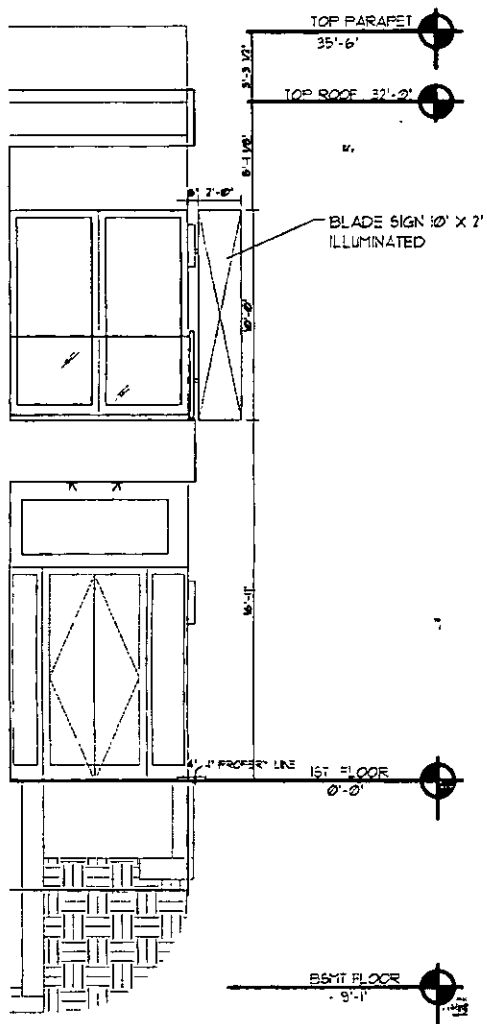
NORTH ELEVATION
