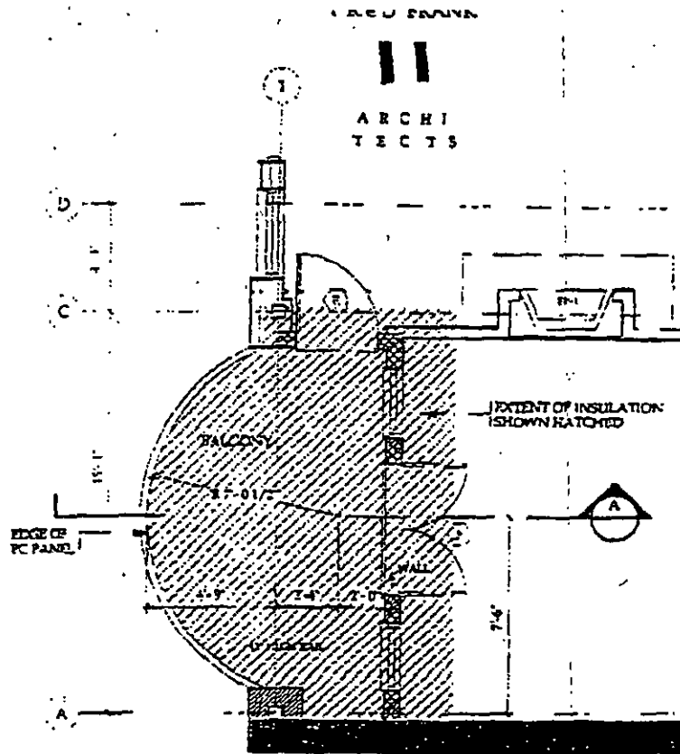
(A) PARTIAL THRD. FLR ARCH. PLAN (4TH/5TH/6TH FLR. SIM.) SCALE: 1/4" = 1'-0"
