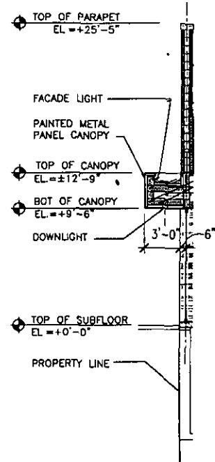
Section
