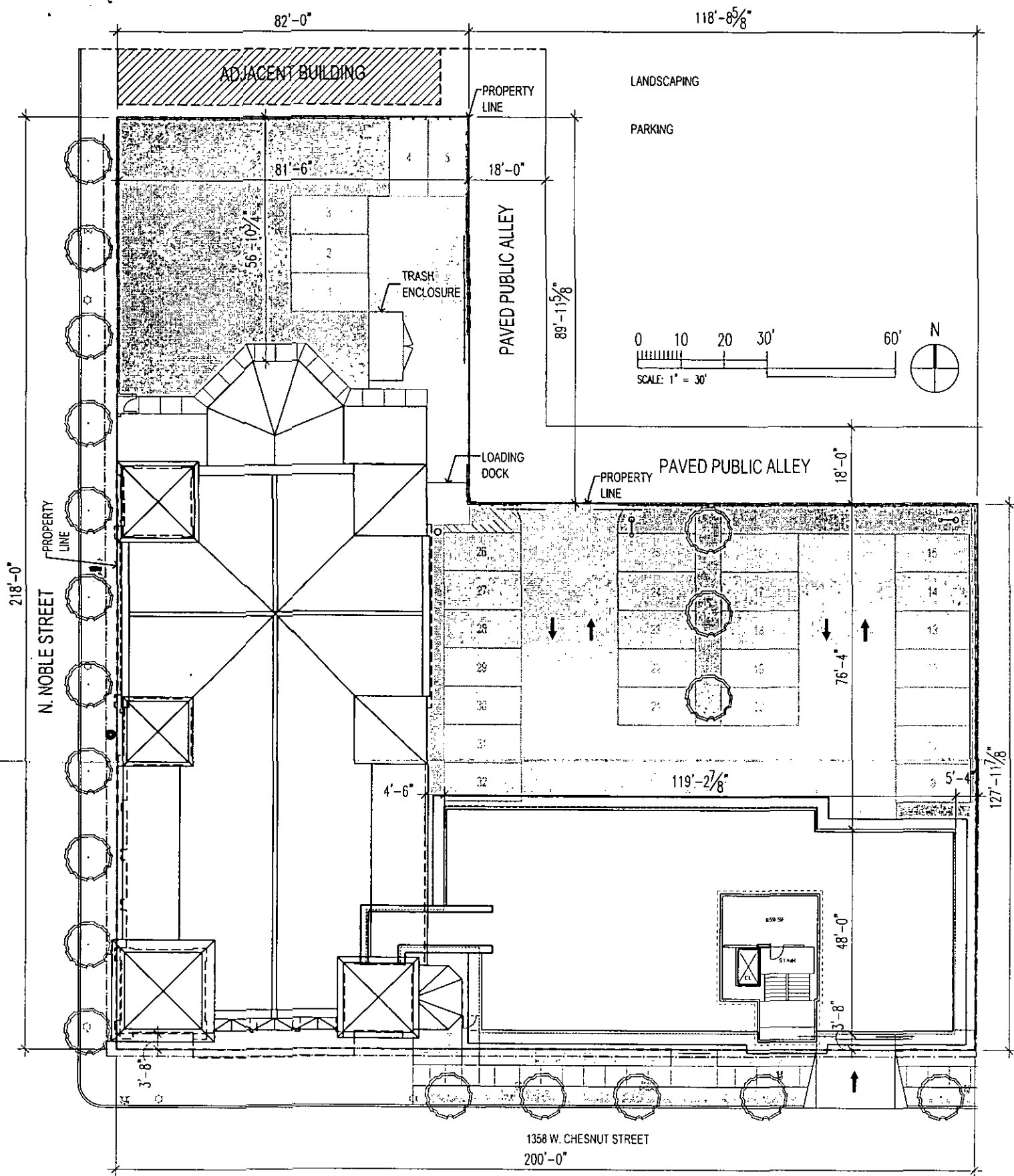
Site Plan - Roof Level
