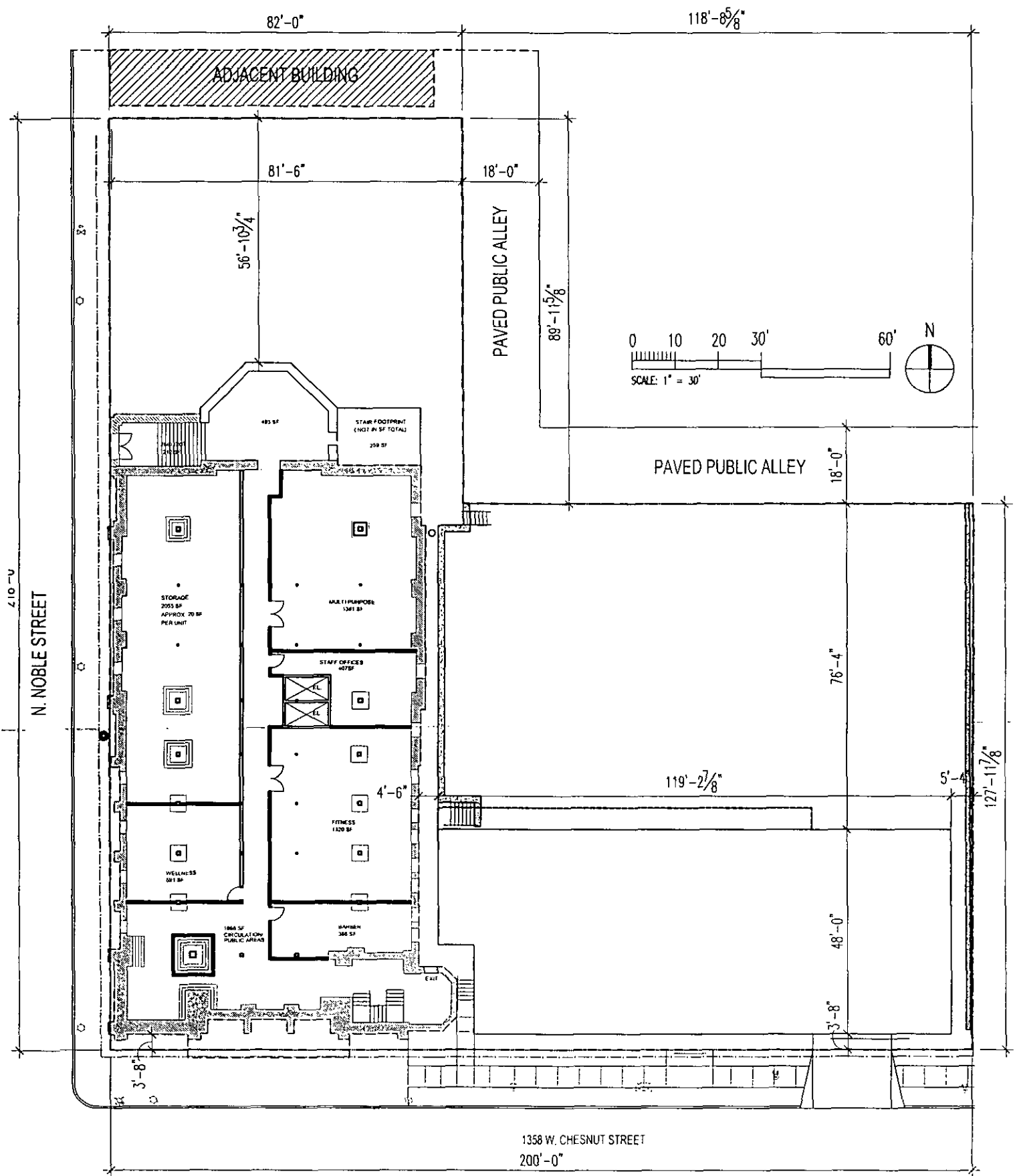
Site Plan Basement Level
