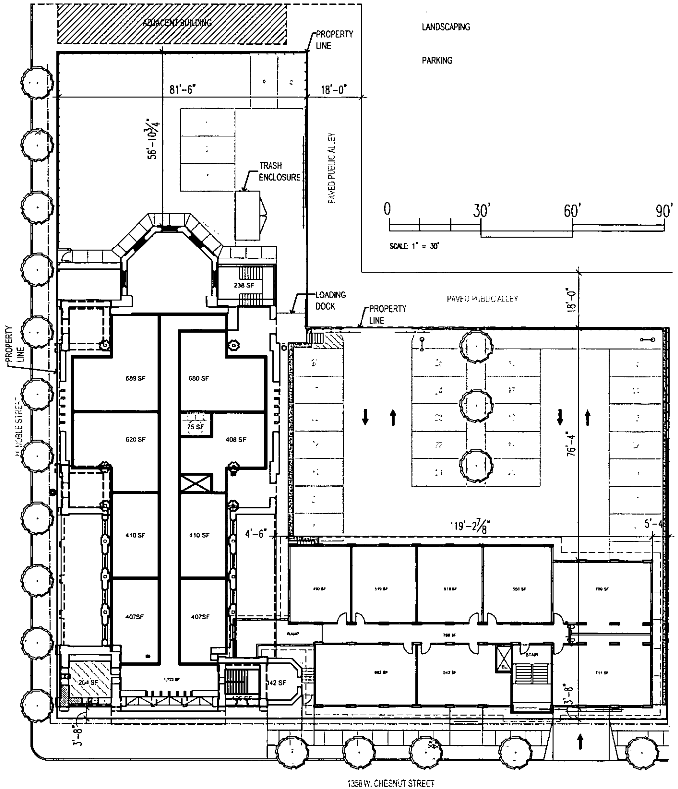
Site Plan Level 04
