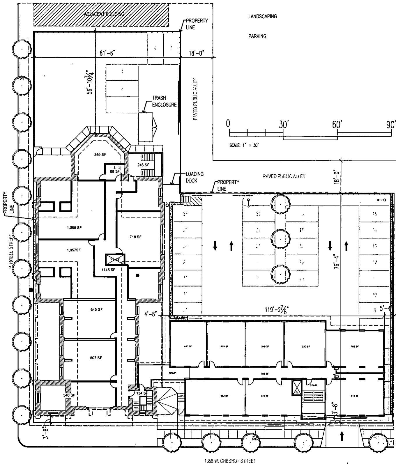
Site Plan Level 05
