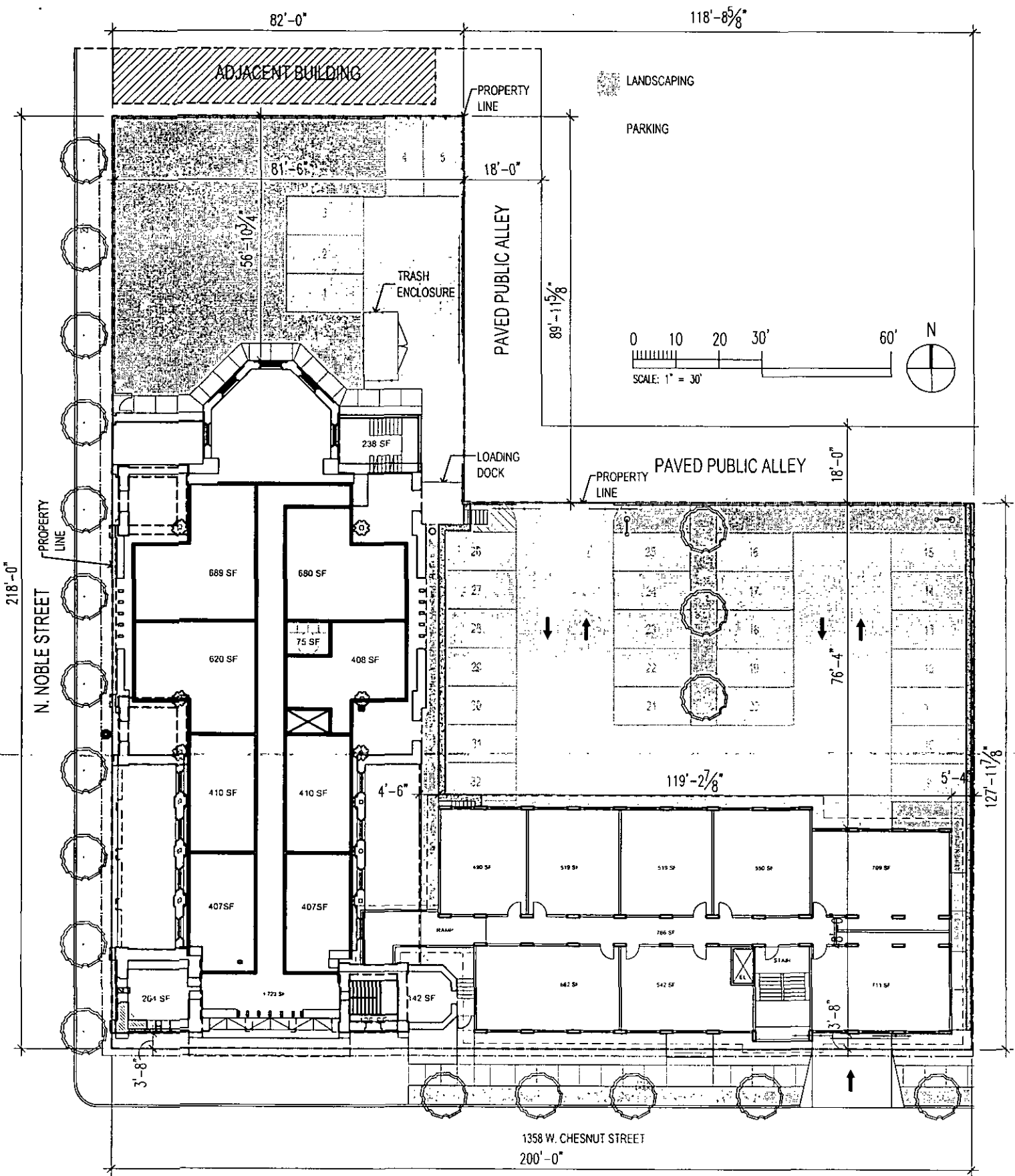
Site Plan Level 04
