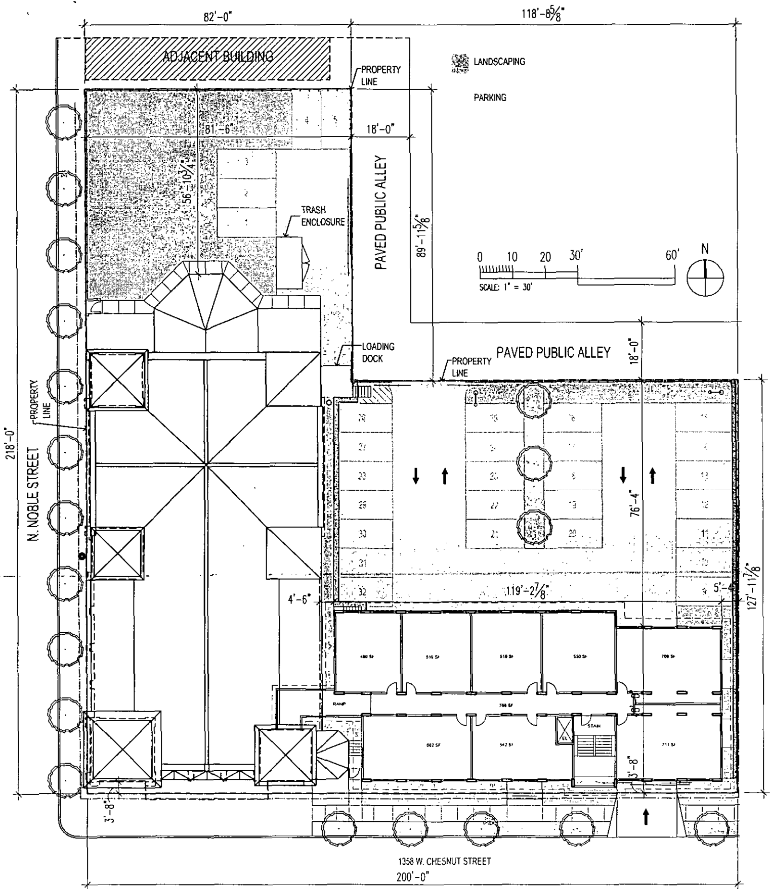
Site Plan Level 06
