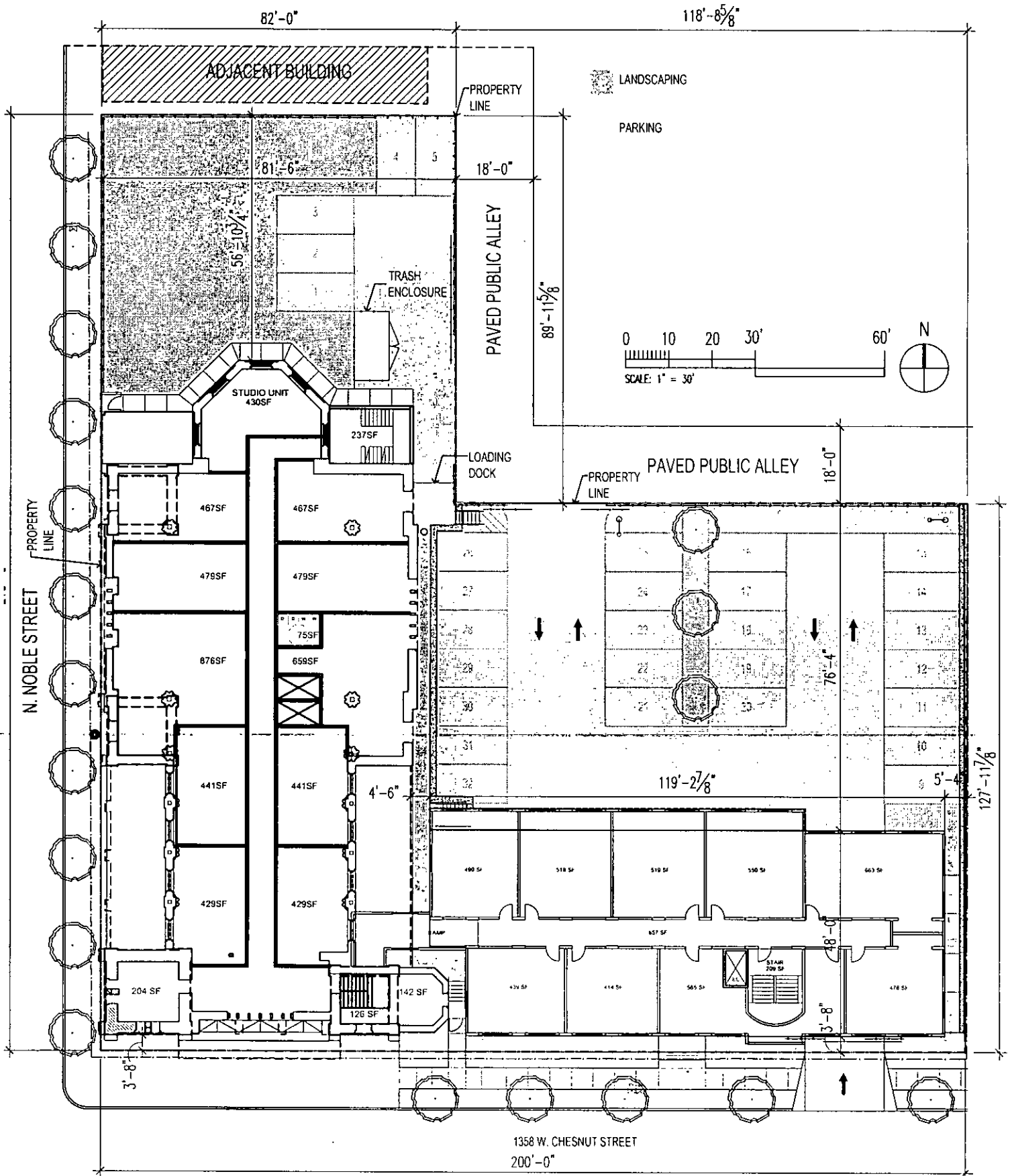
Site Plan Level 02
