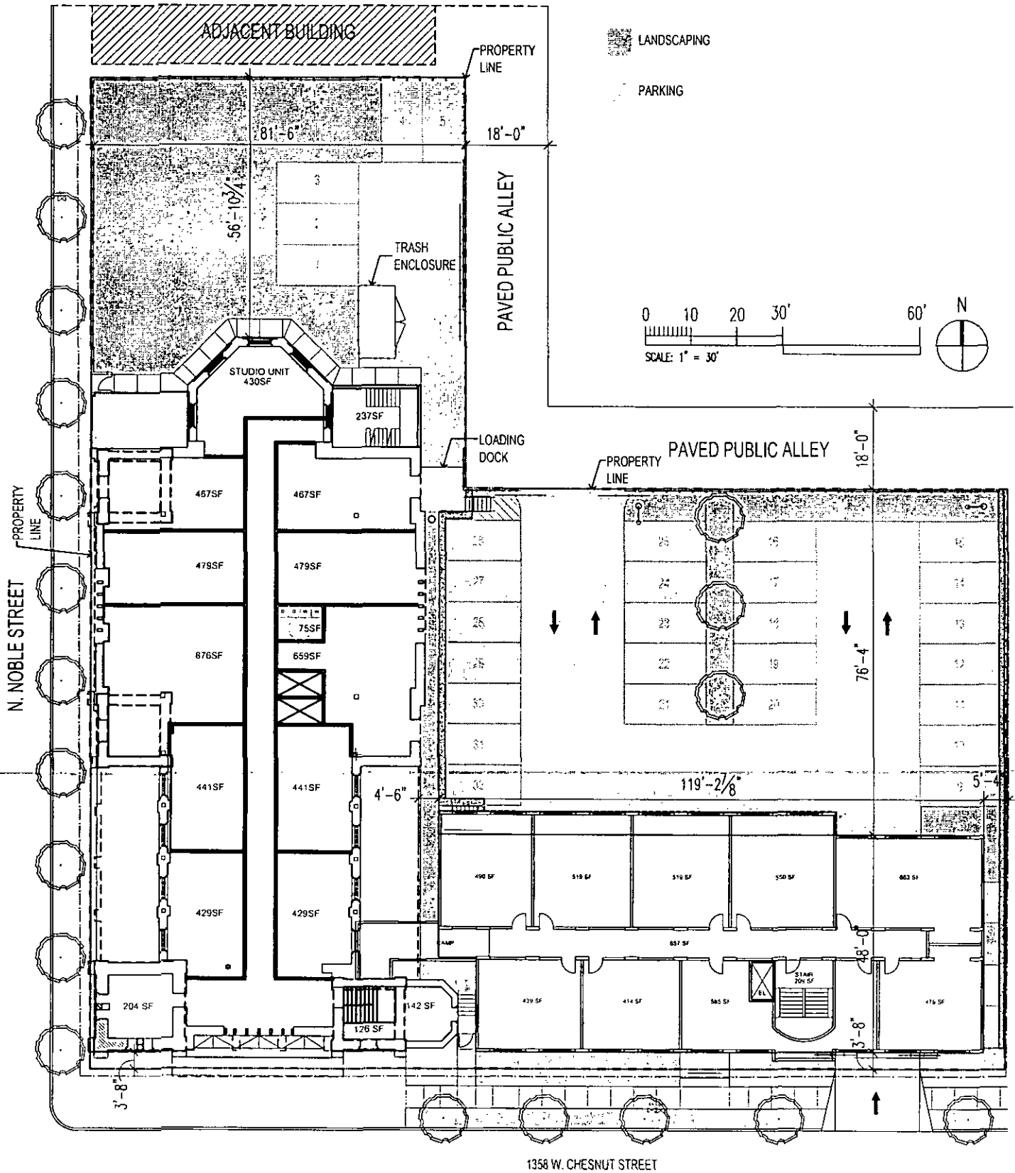
Site Plan Level 03
