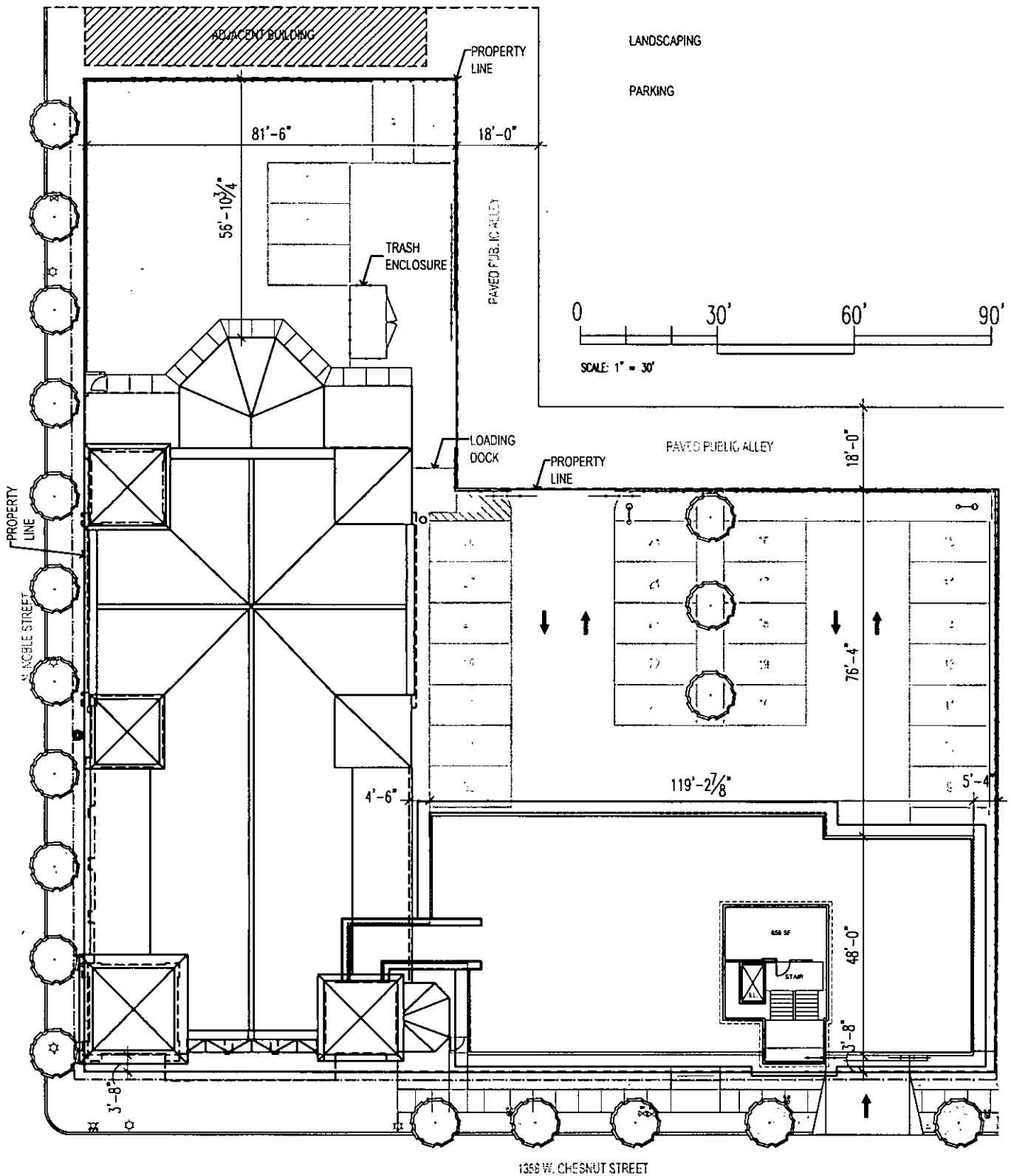
Site Plan - Roof Level
