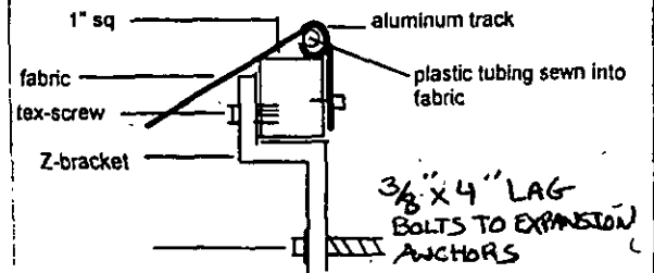
"Z" BRACKET WALL ATTACHMENT DETAIL
