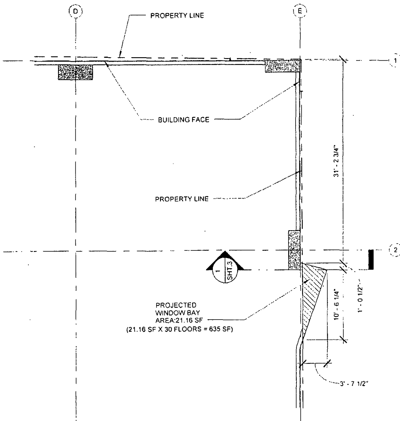
1 ENLARGED PLAN - LEVELS 11-41 WINDOW BAY PROJECTION SCALE 1/8" = 1'-0"
