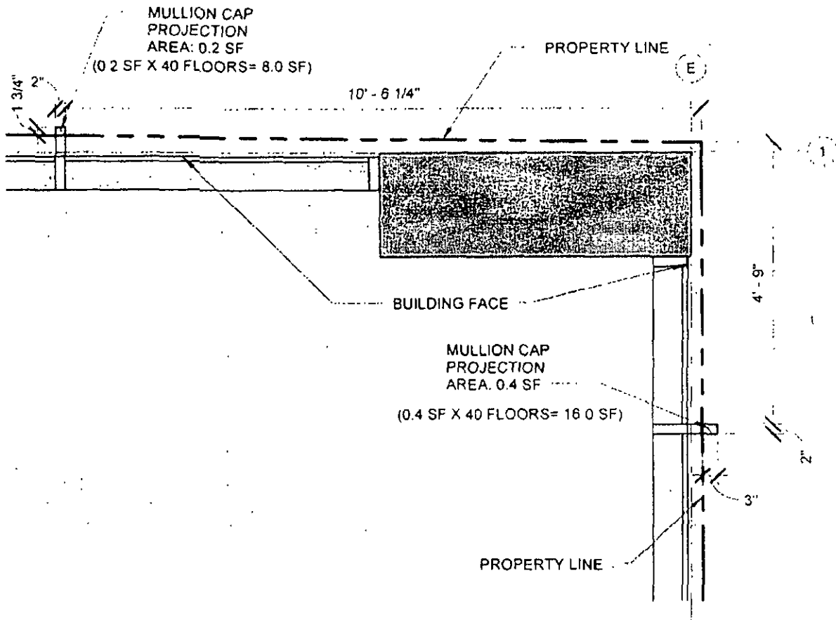
1 ENLARGED PLAN - LEVELS 2 - 41 MULLION CAP PROJECTION 2 SCALE 1/2" = 1'-0"
