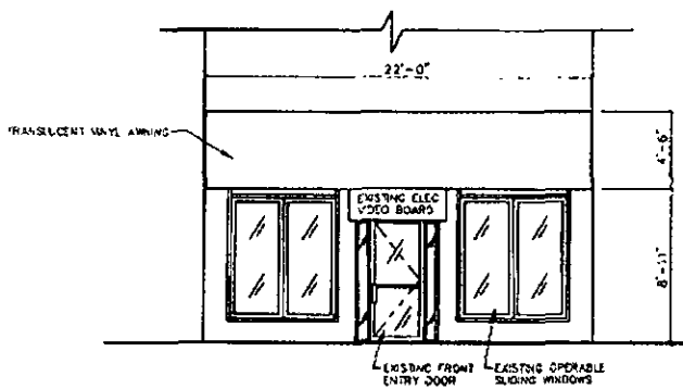
EXISTING ELEVATION
