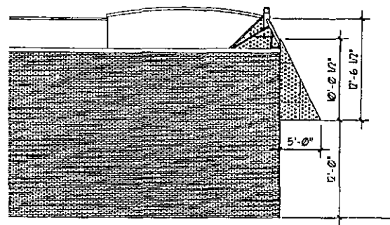
WEST ELEVATION
