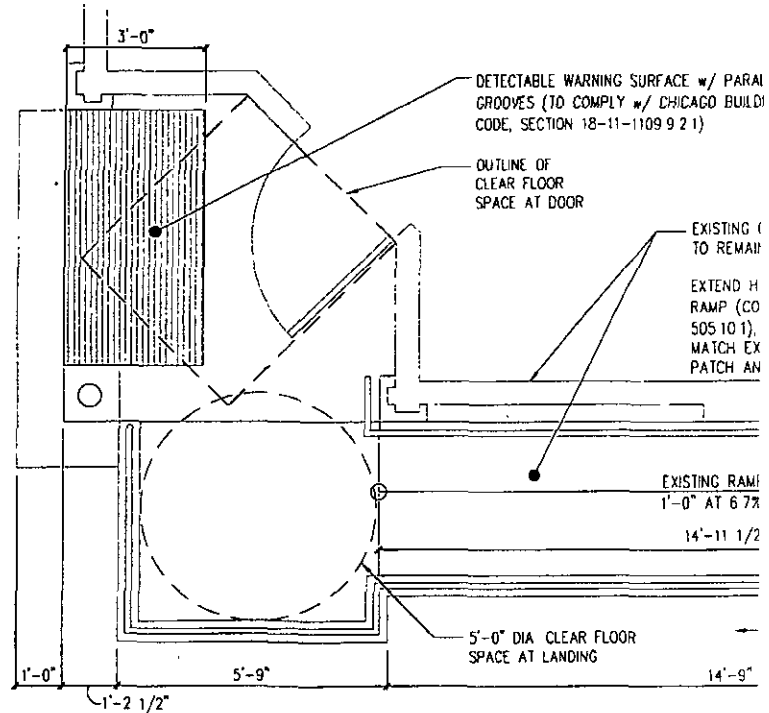
1 RAMP PLAN SCALE: 1/4" = 1'-0"
