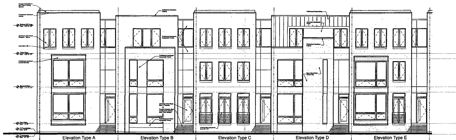
Proposed South Elevation (Partial)
