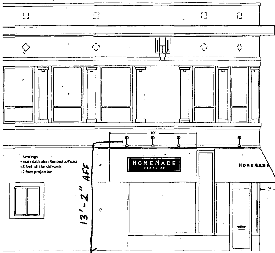
North Elevation
